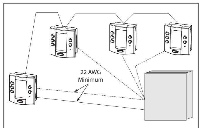
Figure 26. Installing Multiple OneTouch Control Panels
