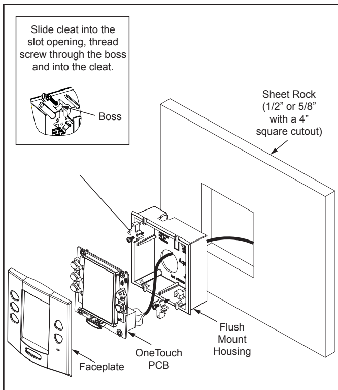
Figure 24. OneTouch Flush Mount Installation
