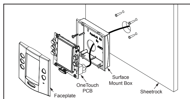
Figure 22. OneTouch™ Surface Mount Installation
