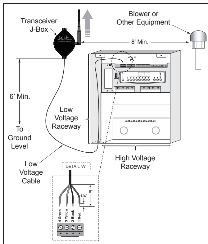
Figure 30. Outdoor Transceiver J-box Installation
