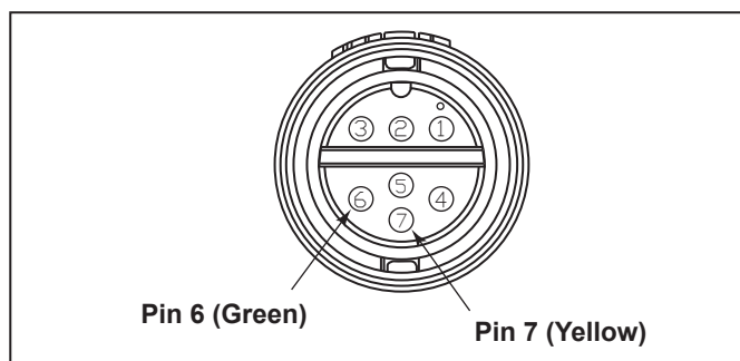
Figure 8. Cable Connector at the Pump Side
