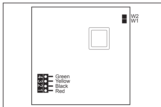
Figure 23. OneTouch PCB - Back View
