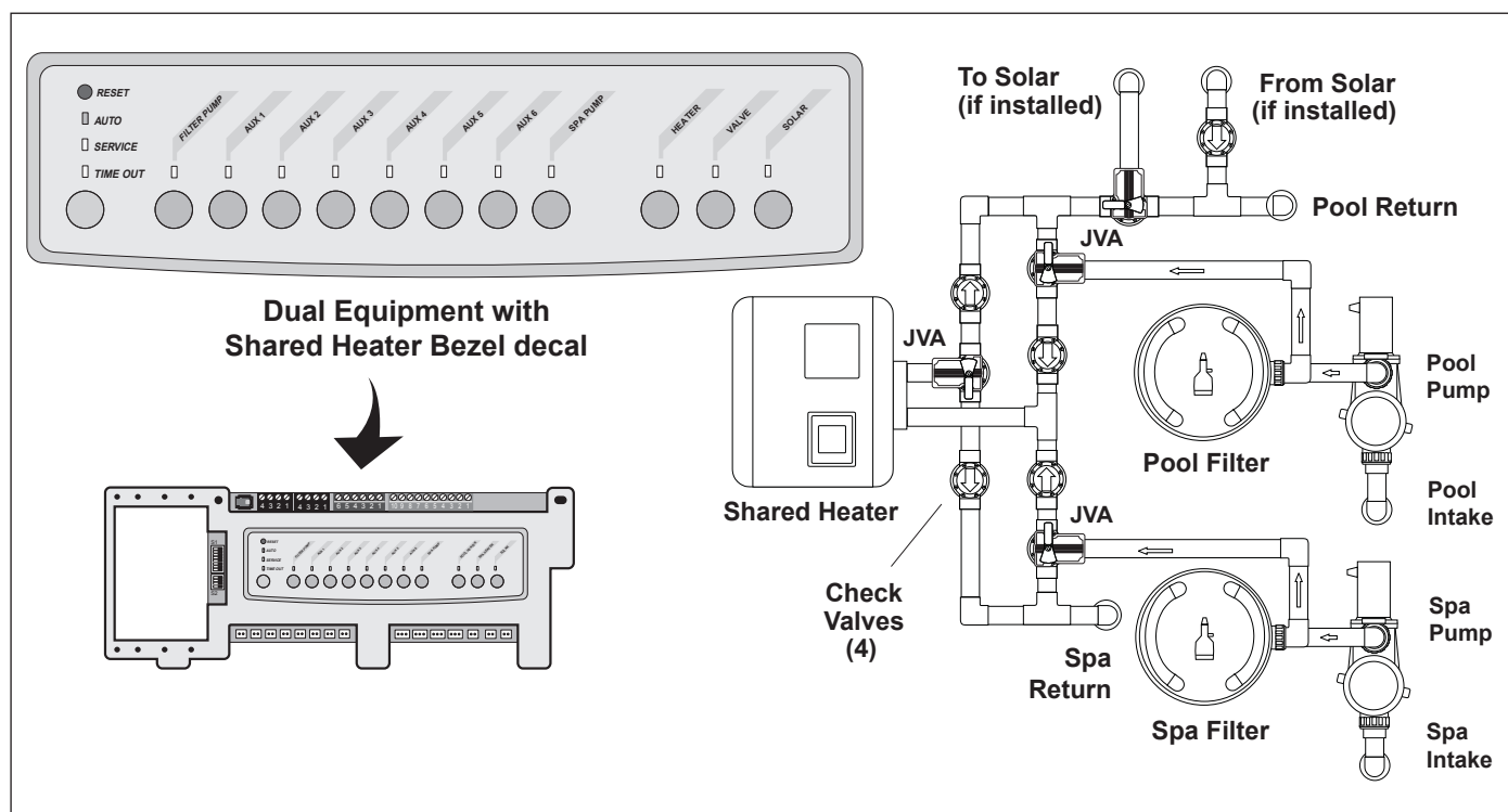
Figure 5. Dual Equipment System with One (1) Heater
