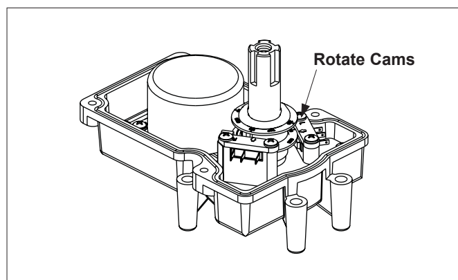
Figure 21. JVA Cam Adjustment
