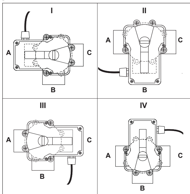
Figure 14. JVA Mounting Positions
