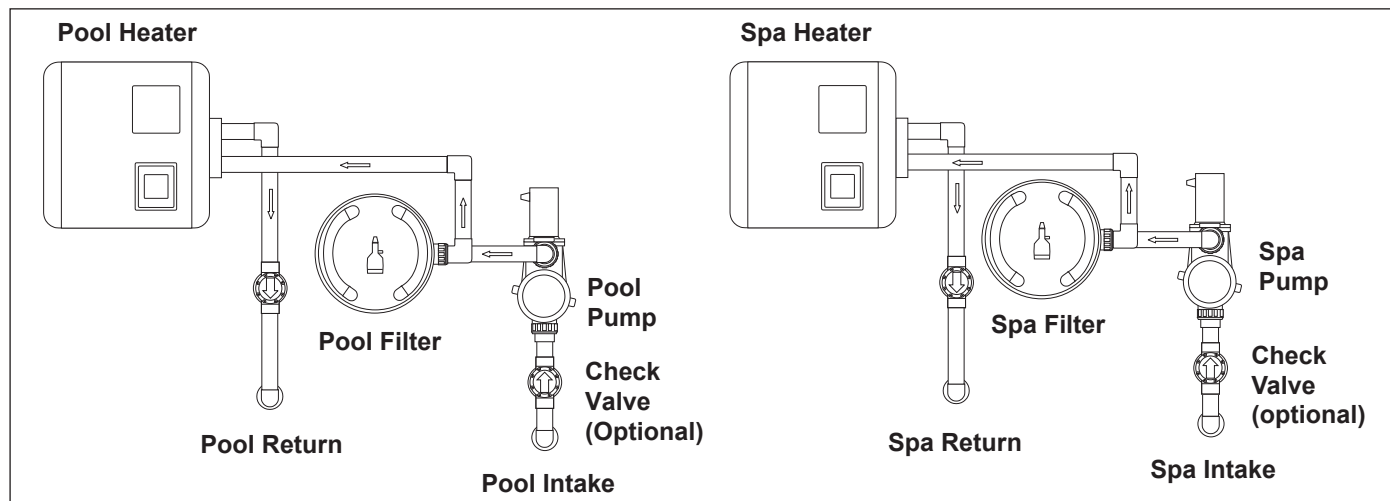
Figure 4. Basic Plumbing for Dual Equipment
