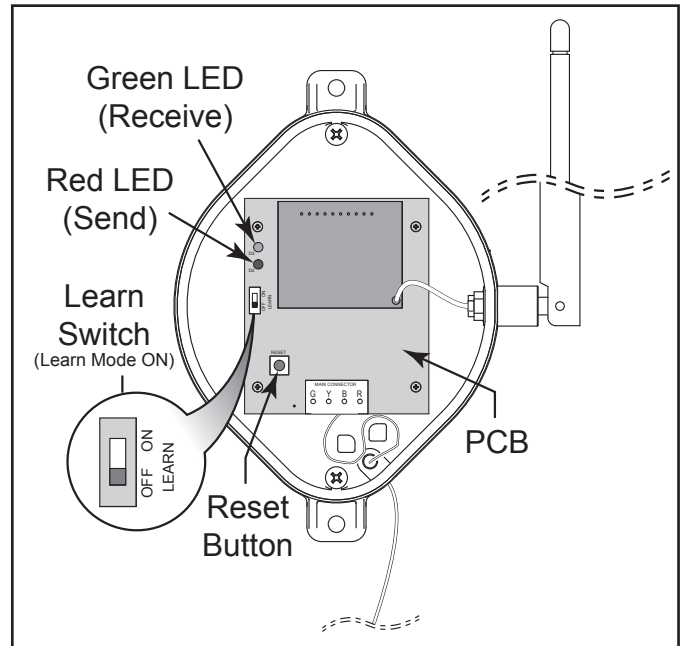
Figure 33. Transceiver J-box PCB Learn Switch
