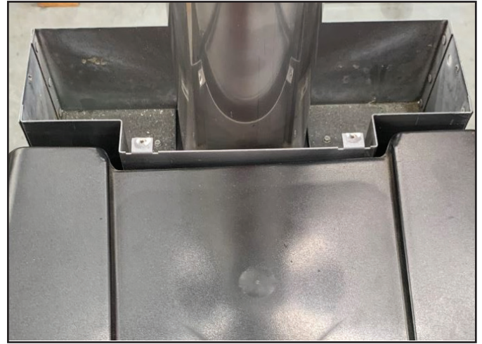
Figure 13. Install Flue into Spigot
