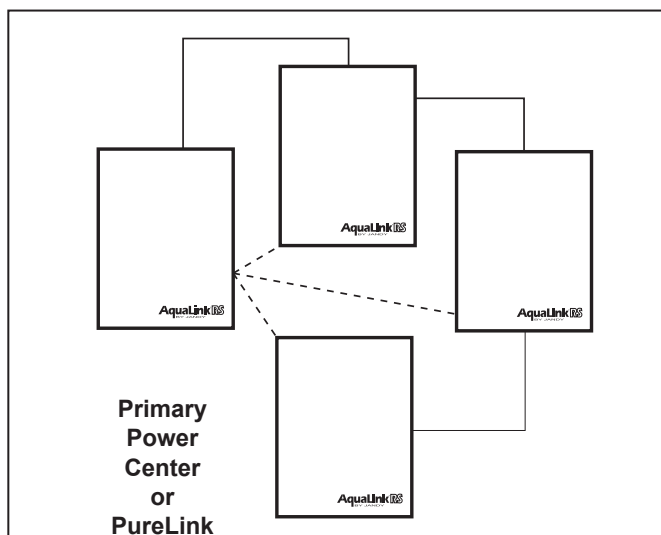
Figure 21. Wiring Multiple Power Centers
